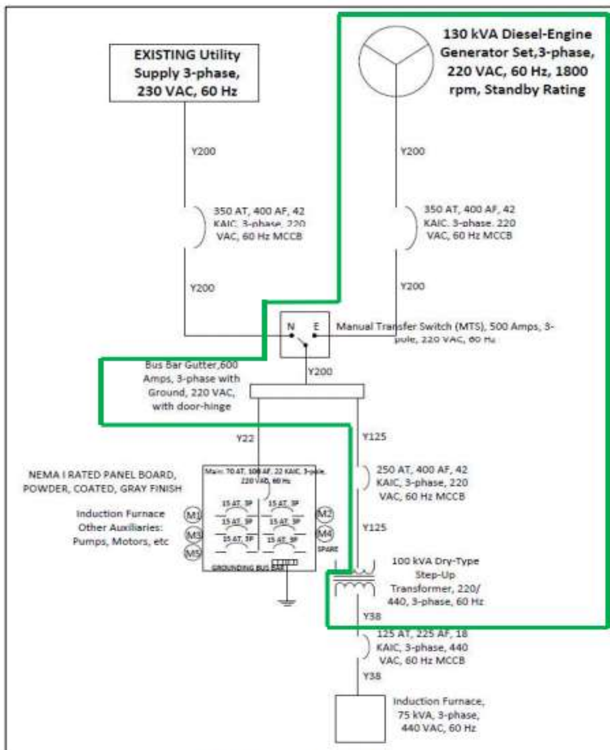
Figure 1: Electrical Diagram
