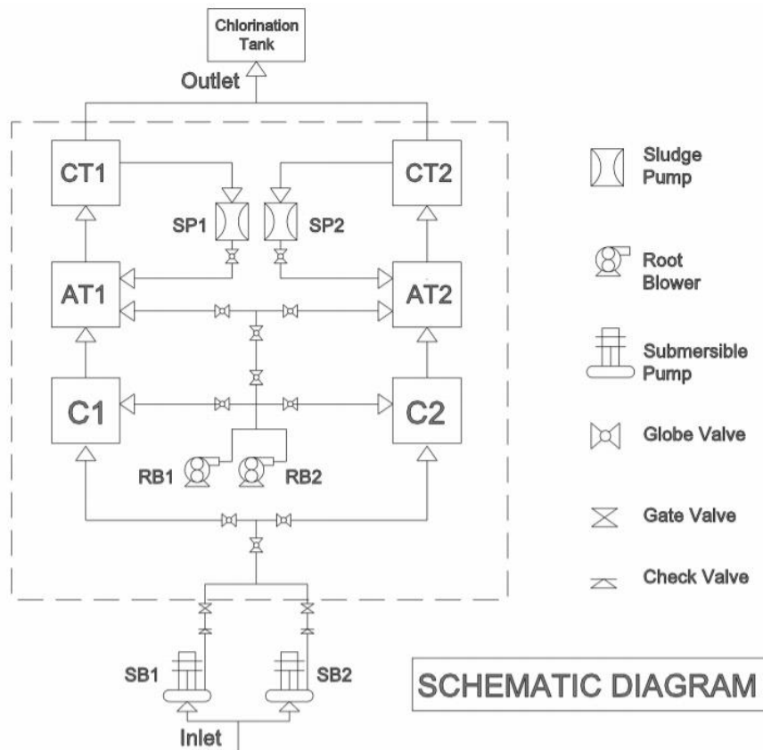
Figure 1. Process Flow for the New/Upgraded STP
