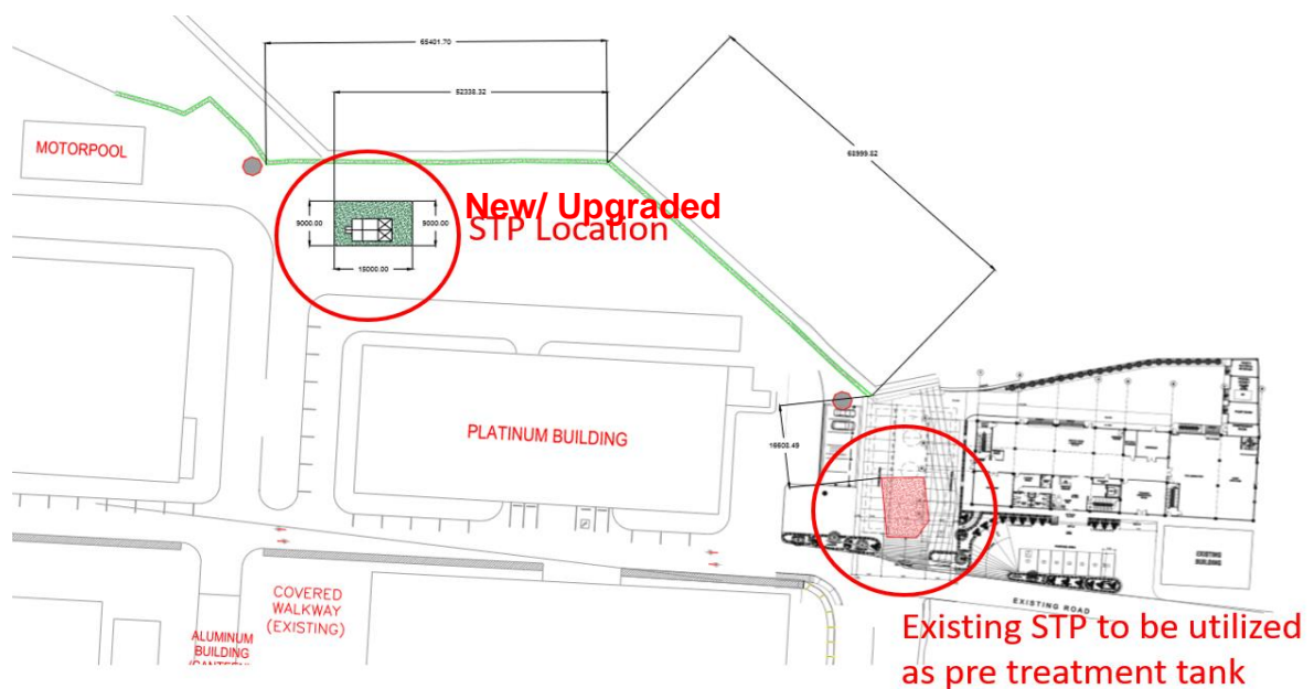
Figure 2. Location Map of the New/Upgraded STP and the existing STP
